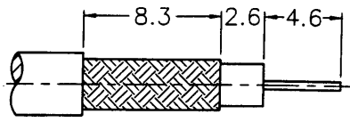
RECOMMENDED CABLE STRIPPING DIM'S (建議剝線尺寸)
