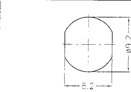
RECOMMENDED MOUNTING HOLE (建議架設孔)
