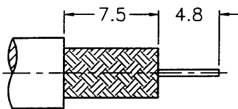
RECOMMENDED CABLE STRIPPING DIM'S (STEP 1) (建議剝線尺寸 步驟一)
