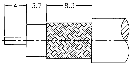
RECOMMENDED CABLE STRIPPING DIM'S (建議剝線尺寸)
