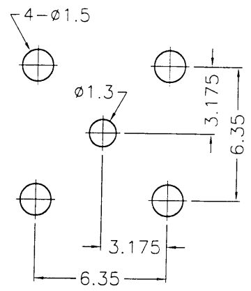
PCB MOUNTING HOLES (印刷电路板架設孔)
