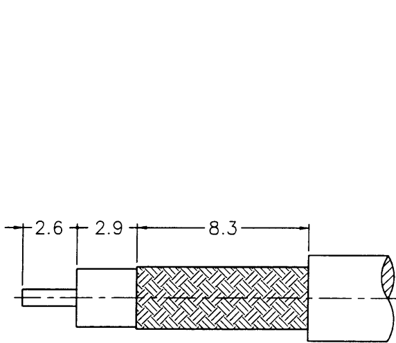
RECOMMENDED CABLE STRIPPING DIM'S (建議剝線尺寸)
