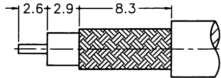
RECOMMENDED CABLE STRIPPING DIM'S (建議剝線尺寸)
