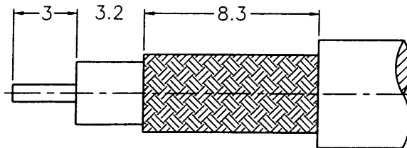
RECOMMENDED CABLE STRIPPING DIM'S (建議剝線尺寸)
