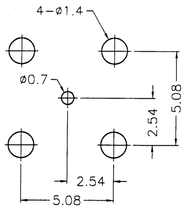
PCB MOUNTING HOLES
