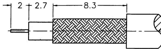
RECOMMENDED CABLE STRIPPING DIM'S (建議剝線尺寸)
