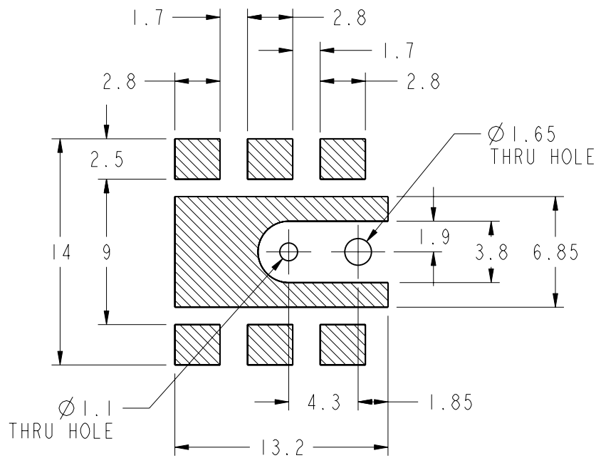
RECOMMENDED PCB LAYOUT (FOR REF ONLY)
